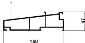
150mm Sill
