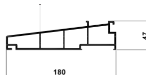
180mm Sill
