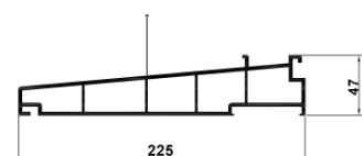
225mm Sill
